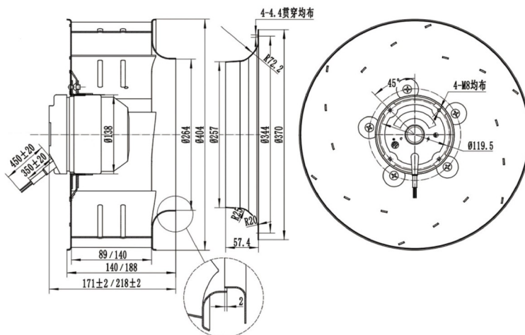
Dimensions Drawing
