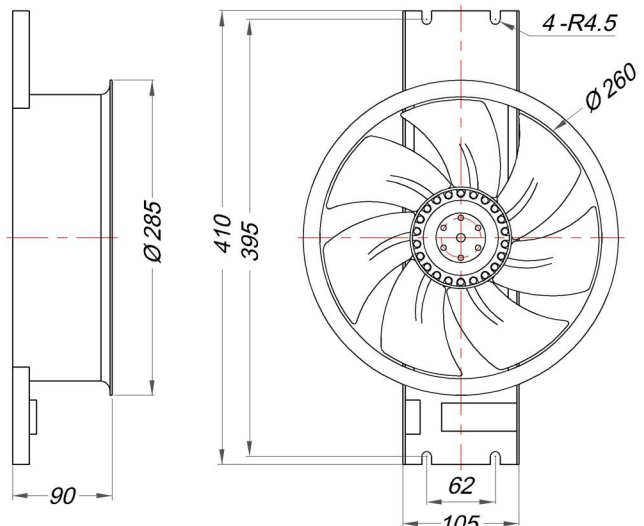
■ Dimensions Drawing
