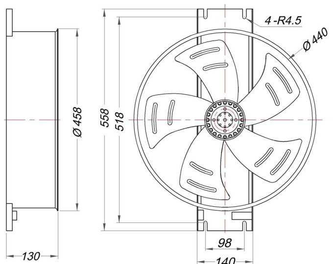
Dimensions Drawing
