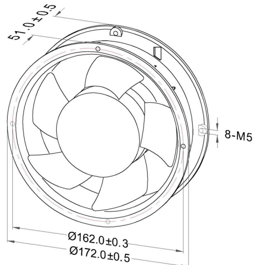
Dimensions Drawing
