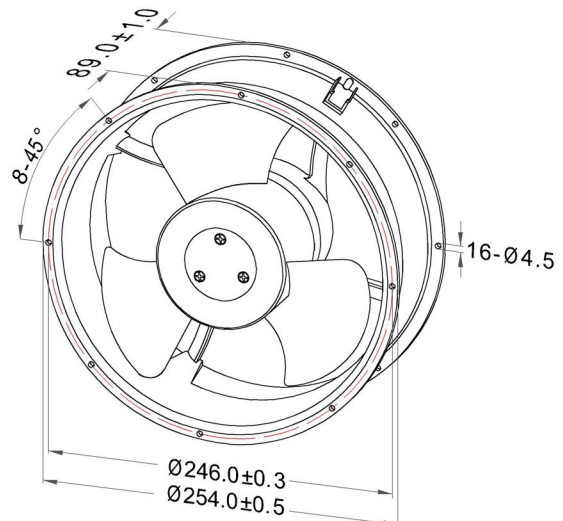
Dimensions Drawing
