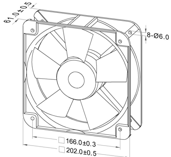
Dimensions Drawing
