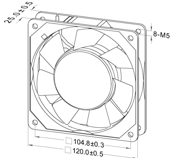
Dimensions Drawing
