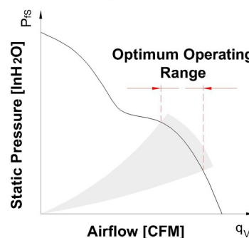
Axial Fan P-Q Characteristic Curve
