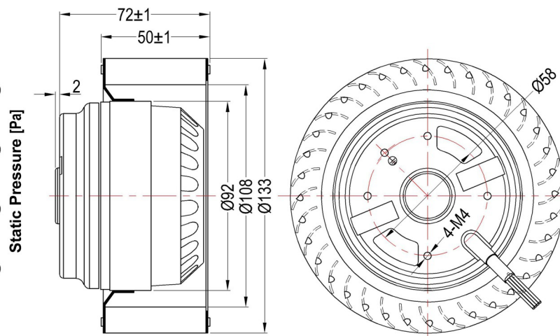
Dimensions Drawing
